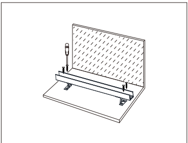
Installation with Adjustable Angle Clip + Aluminum Profile
