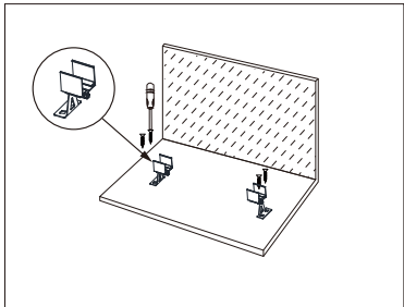
Installation with Adjustable Angle Clip + Aluminum Clip
