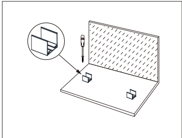
Installation with Aluminum Clip
